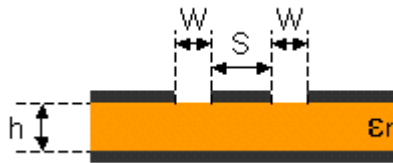
Figure 3-11 Parameters of Coplanar Waveguide with Ground 1
