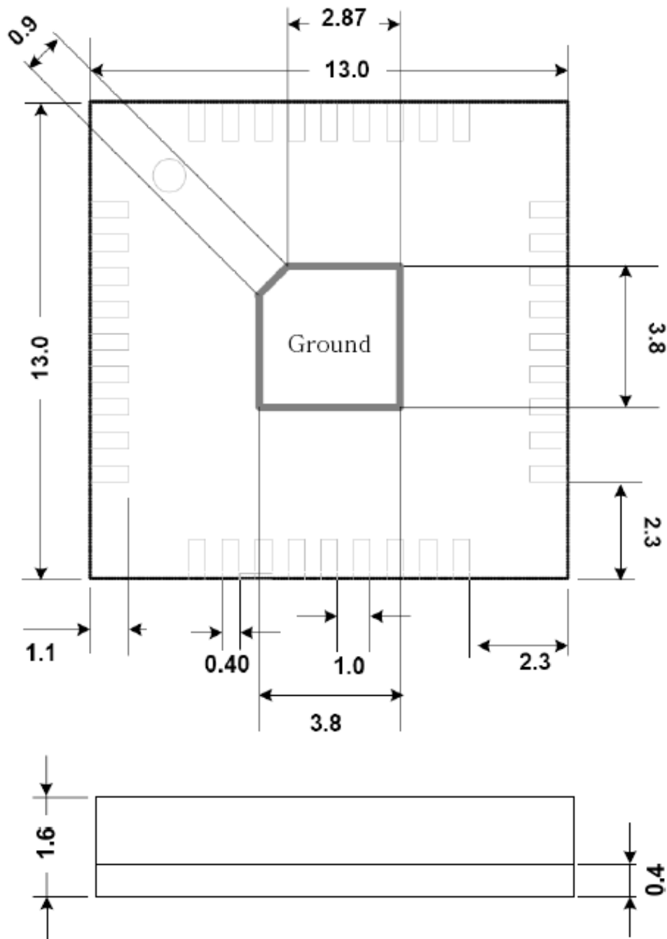
Figure 2-4 HCS-03 Dimensions
