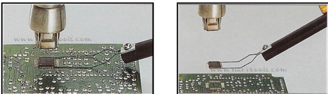
Figure 3-16 Rework Example
